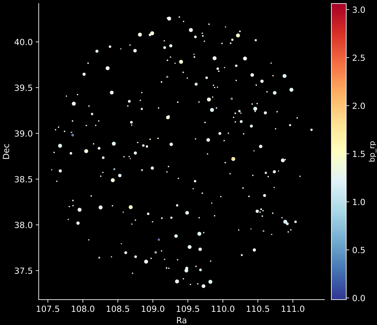
APOGEE DR17 Field: [120-24_btx] Stars: 243
