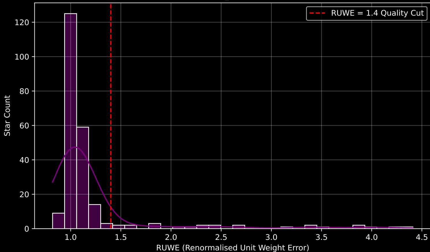
GAPOGEE DR17 Field [120-24_btx] RUWE Distribution (n= 234)
