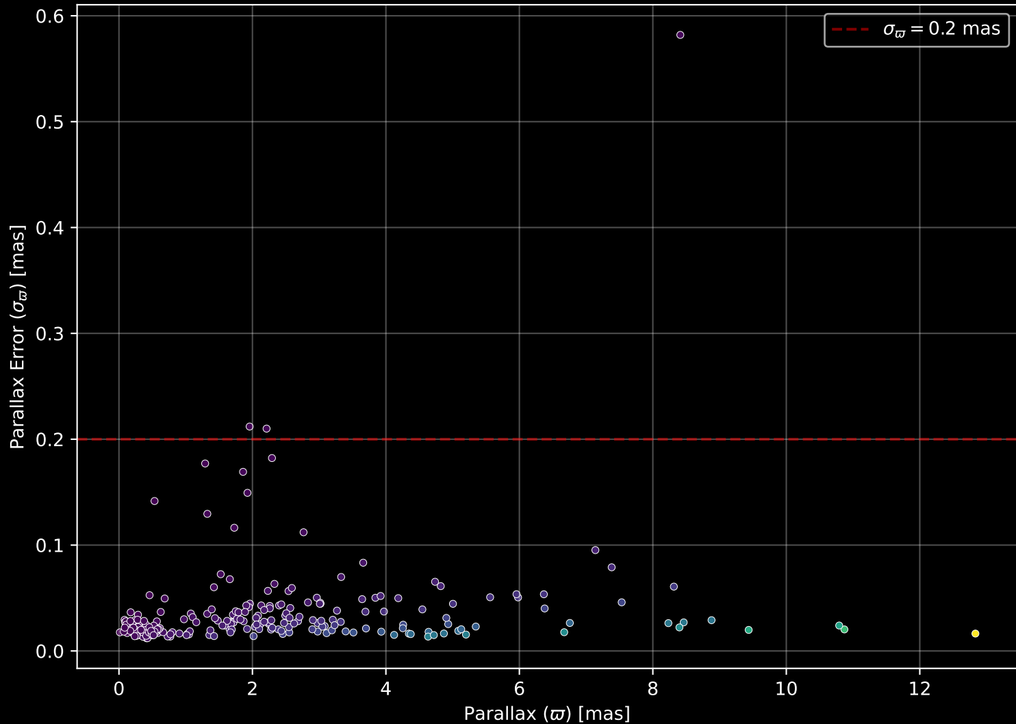
APOGEE DR17 Field: [120-24_btx] Parallax Quality (n= 243)
