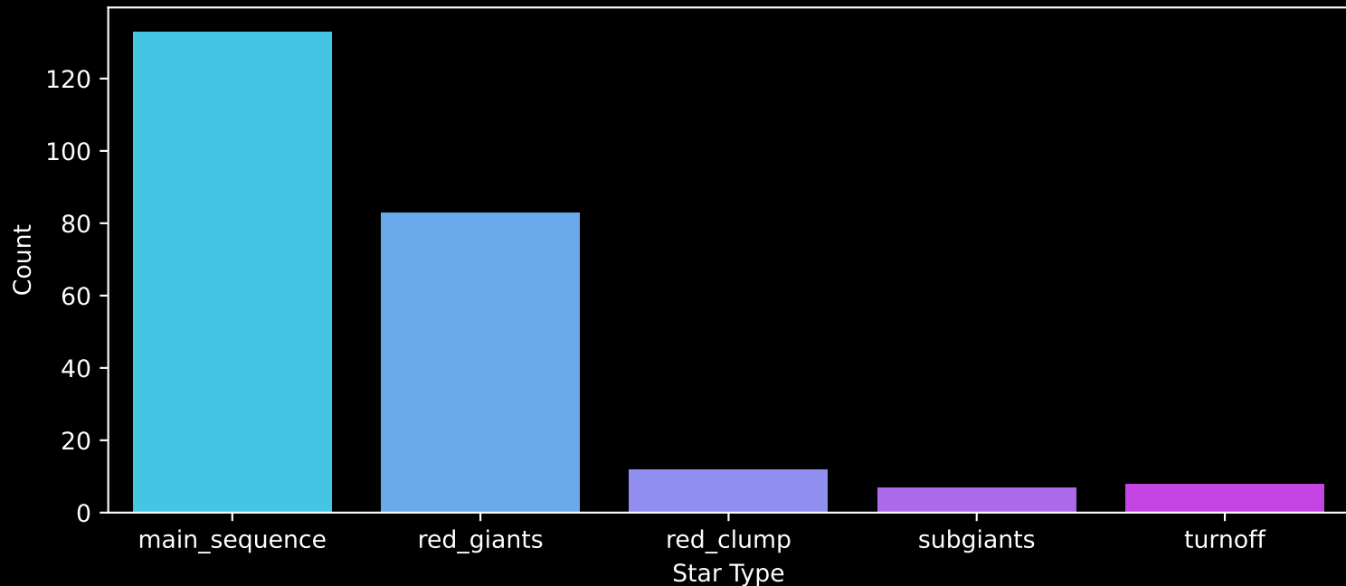
APOGEE DR17 Field: [120-24_btx] Count plot of Star Type
