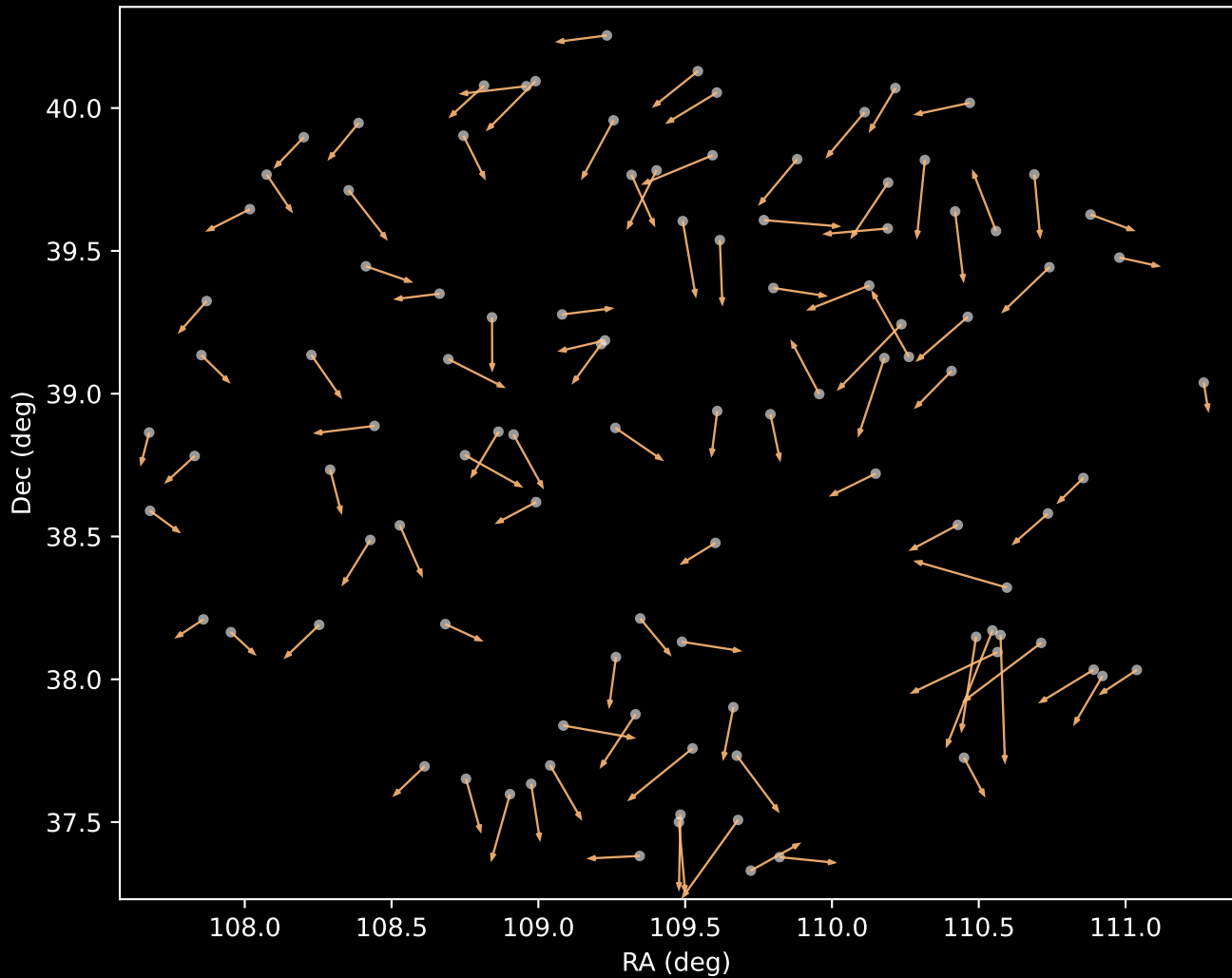
APOGEE DR17 Cluster 3 Proper Motion Vectors (n=103)
