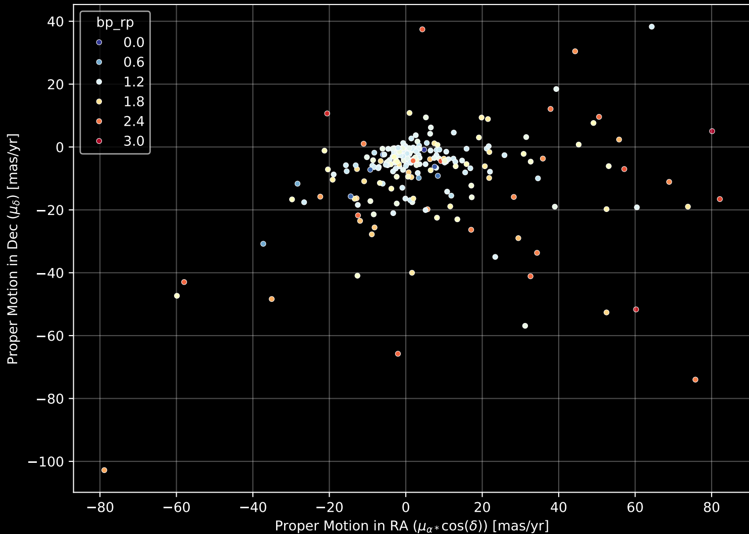
APOGEE DR17 Field: [120-24_btx] Proper Motion Diagram (n= 243)
