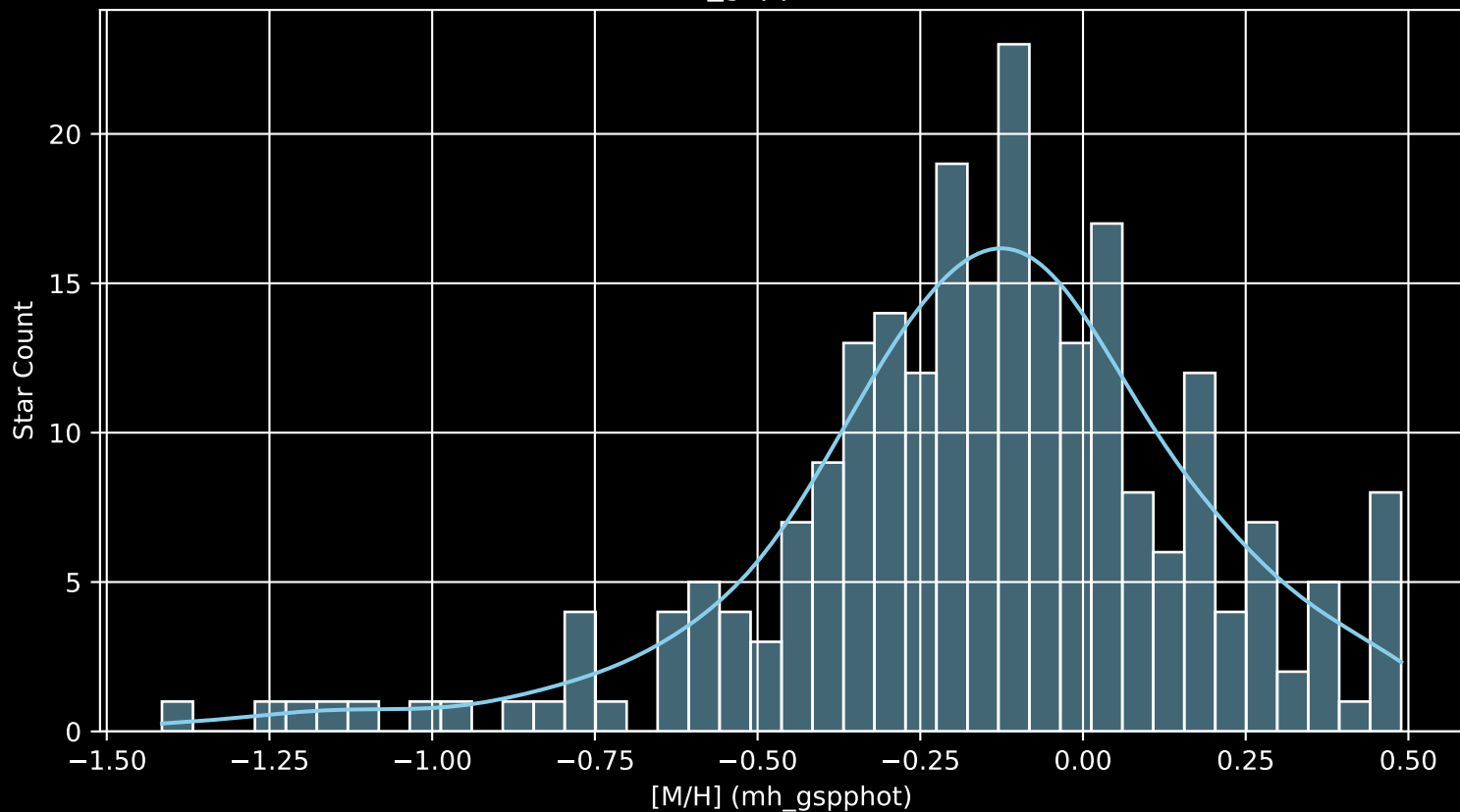
APOGEE DR17 Field: [120-24_btx [M/H] (mh_gspphot) (n= 240)
